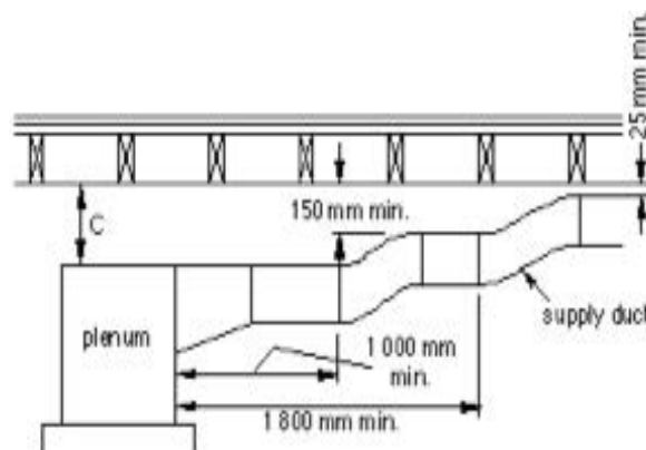
Figure A-6.2.4.10.(3)
