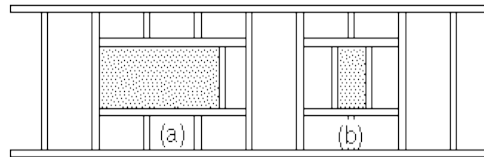
Figure A-9.23.10.6.(2)A. Single Studs at Openings in Non-loadbearing Interior Walls
